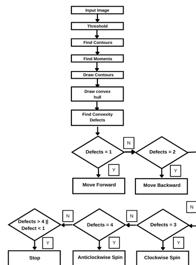
Figure:2 Flowchart
