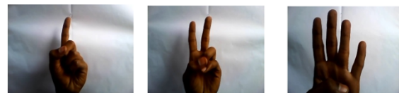
Figure 3: Input Images
