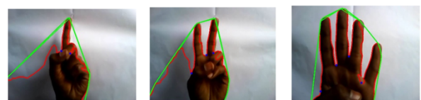
Figure 4: Output Images
